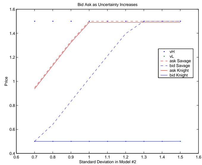
Figure 5: Bid and Ask as Uncertainty Increases
